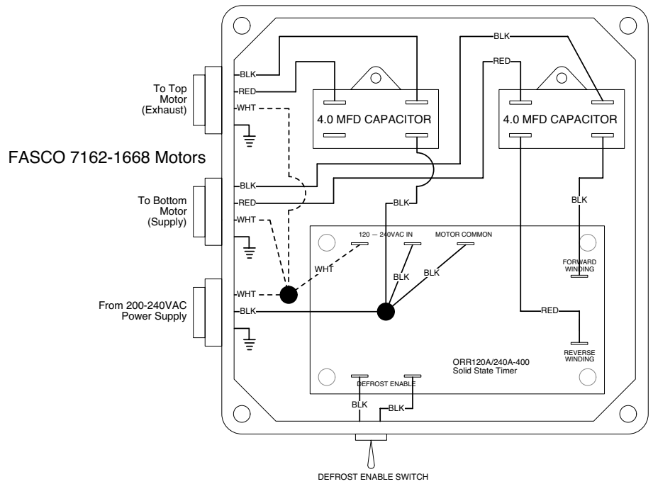
Figure 1 RA402 Wiring Diagram as of November, 2002
